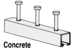
Concrete Insert With 1/2" x 3" studs PS 5000T
