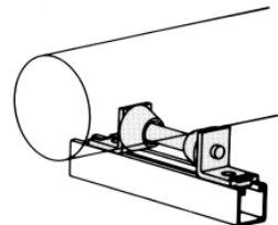
Pipe Roller Support PS 1901 1"-8" pipe sizes PS 1902 1"-12" pipe sizes
