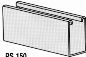
PS 150 1 5/8" x 2 7/16" x 12 ga.
