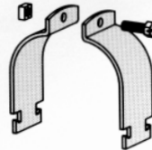
PS 1000 EMT Conduit Clamp 1/2"-2" conduit sizes PS 1100 Standard Pipe Clamp (GRC and IMC) 3/8"-10" pipe sizes PS 1200 O.D. Tubing Clamp 1/4"-8 5/8" O.D. sizes PS 1300 Universal Pipe Clamp for EMT, IMC & GRC 1/2"-2" pipe sizes
