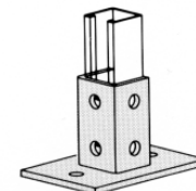
Post Base PS 3025 for PS 200 & 210 PS 2064 for PS 200 2T3 PS 3013 for PS 200 & 210 PS 3029 for PS 200 2T3 PS 3064 for PS 200 2T3
