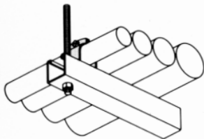
PS 1000 EMT Conduit Clamp 1/2"-2" conduit sizes PS 1100 Standard Pipe Clamp (GRC and IMC) 3/8"-10" pipe sizes PS 1200 O.D. Tubing Clamp 1/4"-8 5/8" O.D. sizes PS 1300 Universal Pipe Clamp for EMT, IMC & GRC 1/2"-2" pipe sizes
