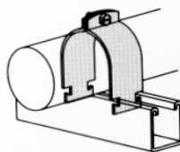
PS 1000 EMT Conduit Clamp 1/2"-2" conduit sizes PS 1100 Standard Pipe Clamp (GRC and IMC) 3/8"-10" pipe sizes PS 1200 O.D. Tubing Clamp 1/4"-8 5/8" O.D. sizes PS 1300 Universal Pipe Clamp for EMT, IMC & GRC 1/2"-2" pipe sizes
