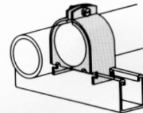
Clamp With Cushions PS 1400 Assembly Includes Clamp and Thermoplastic Cushions 3/8"-2 1/2" O.D. sizes
